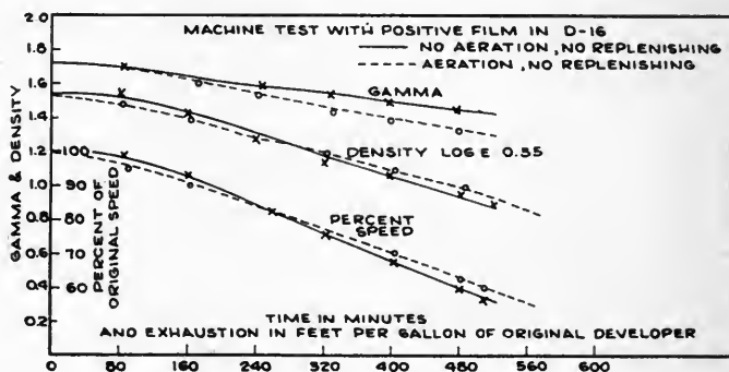
FIG. 8. Effect of exhaustion of D-16 developer, with and without aeration, when in use in a motion picture processing machine.
